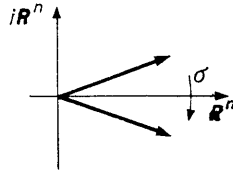
Fig. 118. The complex conjugate
