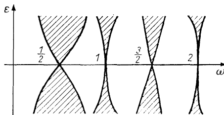
Fig. 209. The region of instability for Eq. (4)
