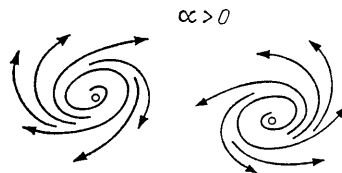
Fig. 138. Unstable foci
