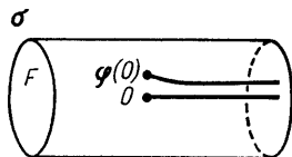
Fig. 170. Indefinite forward extensibility of the solution
