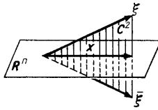
Fig. 130. The real part of a complex eigenvector belongs to an invariant real plane
