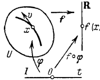
Fig. 84. The derivative of the function f in the direction of the vector \mathbf{v}
