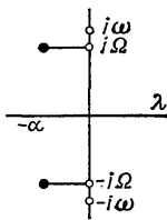
Fig. 187. The eigenvalues of the equation of the pendulum with friction
