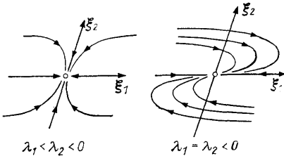
Fig. 133. Stable nodes
