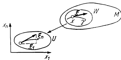
Fig. 250. The coordinates of a tangent vector
