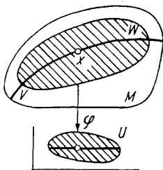
Fig. 246. A submanifold
