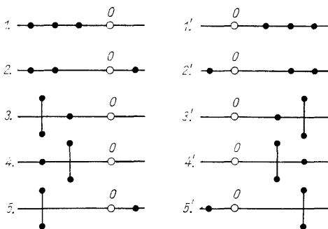
Fig. 142. The eigenvalues of a real operator A: R^3 \rightarrow R^3 . Robust cases
