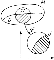
Fig. 239. An open subset
