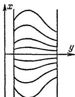
Fig. 39. The integral curves of a linear equation
