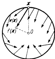
Fig. 264. A mapping of a disk into itself
