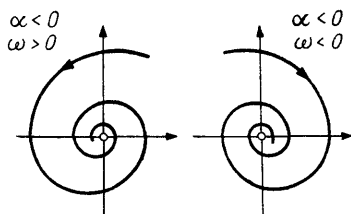
Fig. 123. Stable foci
