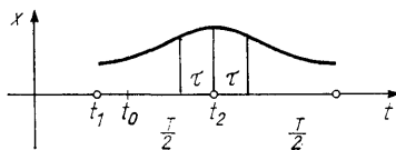
Fig. 104. Extension of a solution of Newton's equation using reflections
