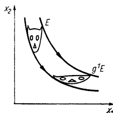
Fig. 47. A hyperbolic rotation
