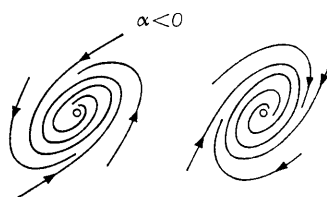
Fig. 136. Stable foci
