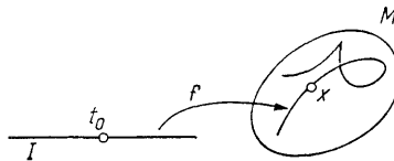
Fig. 244. A curve on a manifold M
