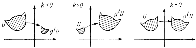
Fig. 114. The behavior of areas under the phase flow transformations of the pendulum equation
